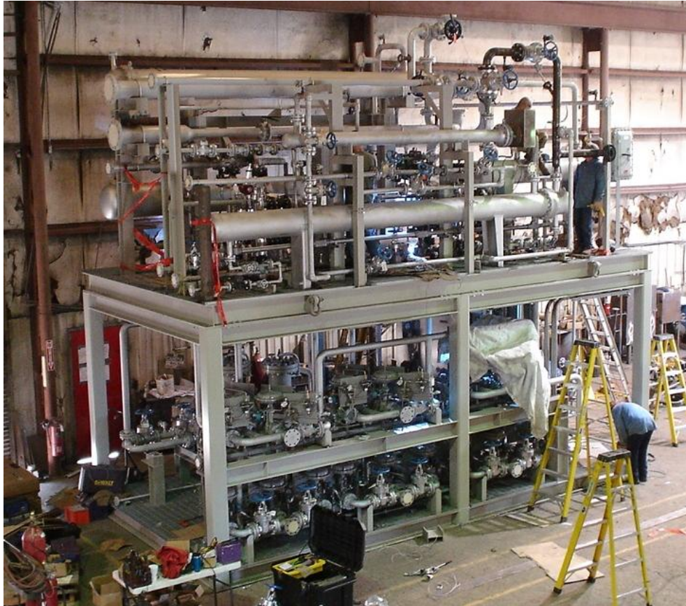
Compact Dehydration Skid for installation at a petrochemical plant with very limited space
